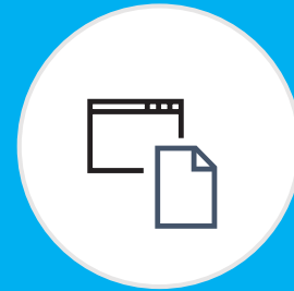
SharePoint Server 2019
