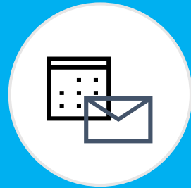
Exchange Server 2019
